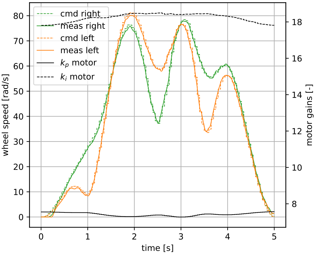
Wheel Speeds
